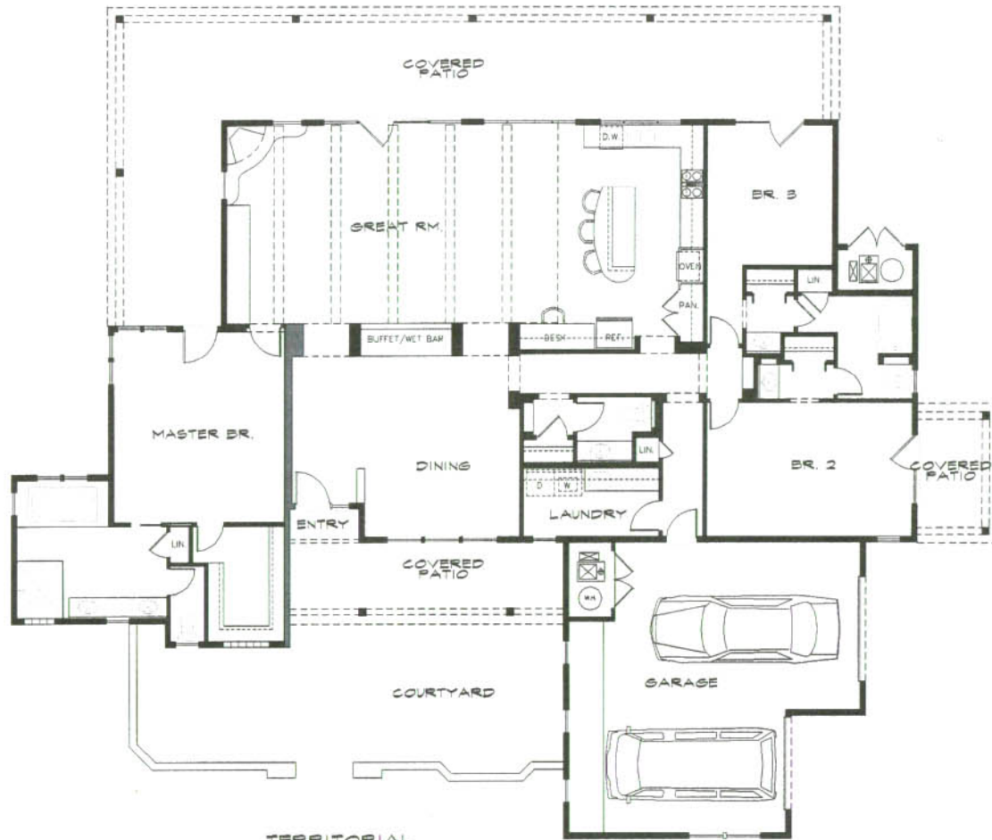
TERRITORIAL FLOOR PLAN
